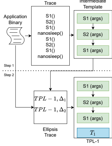
Fig. 2. Ellipsis template creation.
